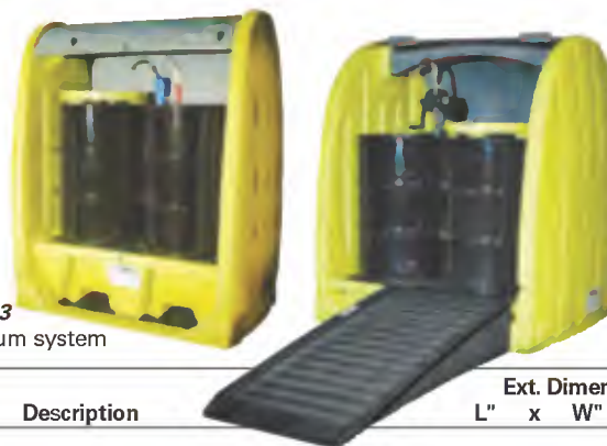
SI740 4-Drum system with optional ramp
